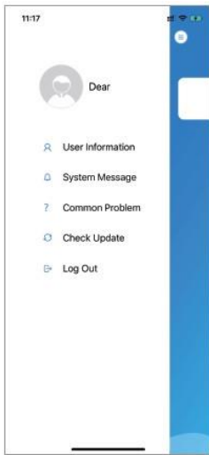
Fig.5 The left-handmenu
